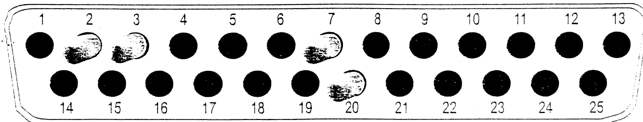
DB 25 Male Connector (mating end)
