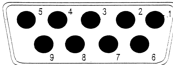
DB 9 Female Connector (mating end)
