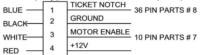
Ticket Dispenser Connection Diagram
