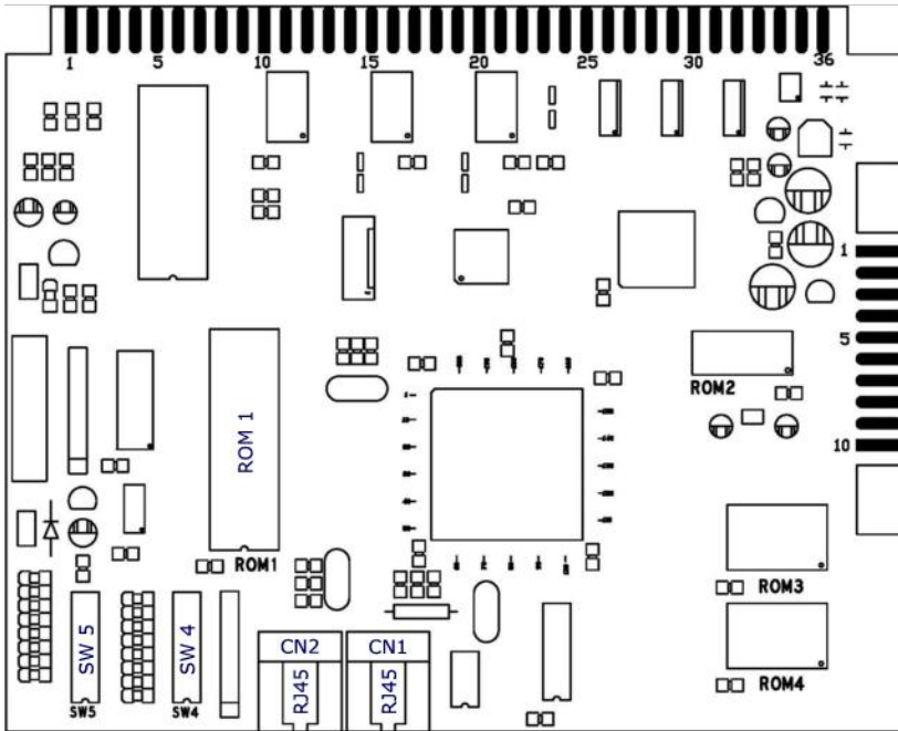
Hopper Connection Diagram
